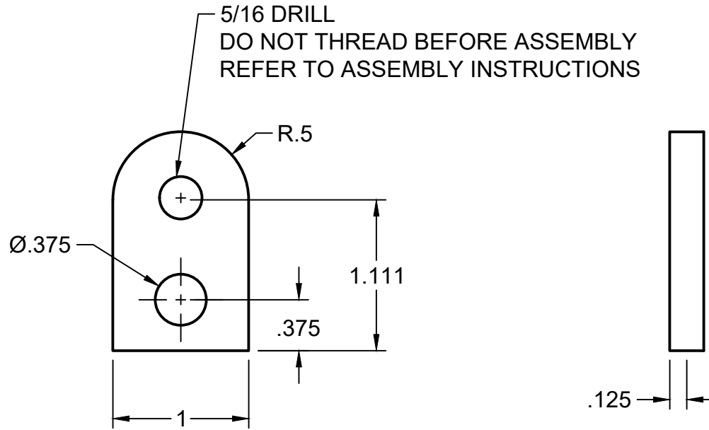
ITEM 14 - LEFT THREAD EXTENSION
