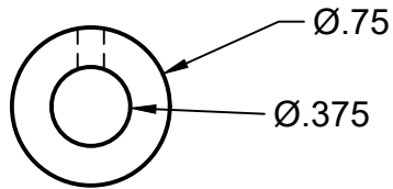
ITEM 5 - LEAD SCREW COLLAR
