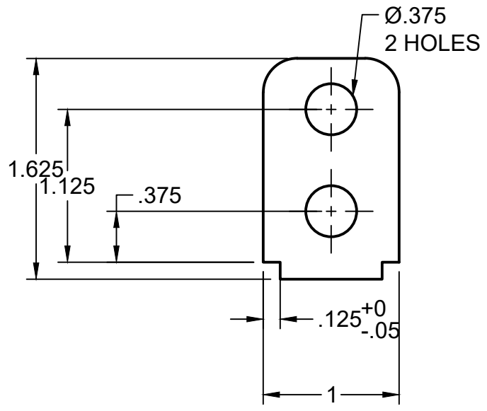
ITEM 1 - SUPPORT
