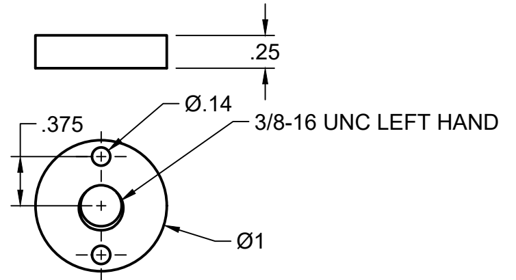
ITEM 7 - RIGHT THREAD INSERT
