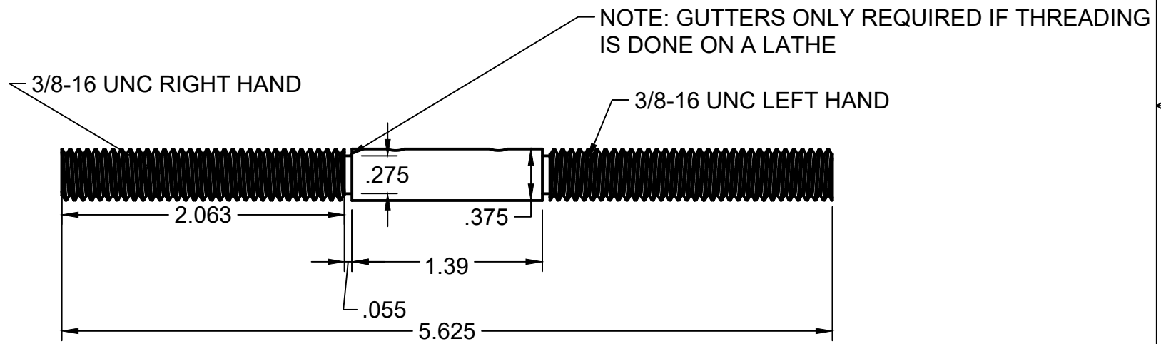
ITEM 4 - LEAD SCREW
